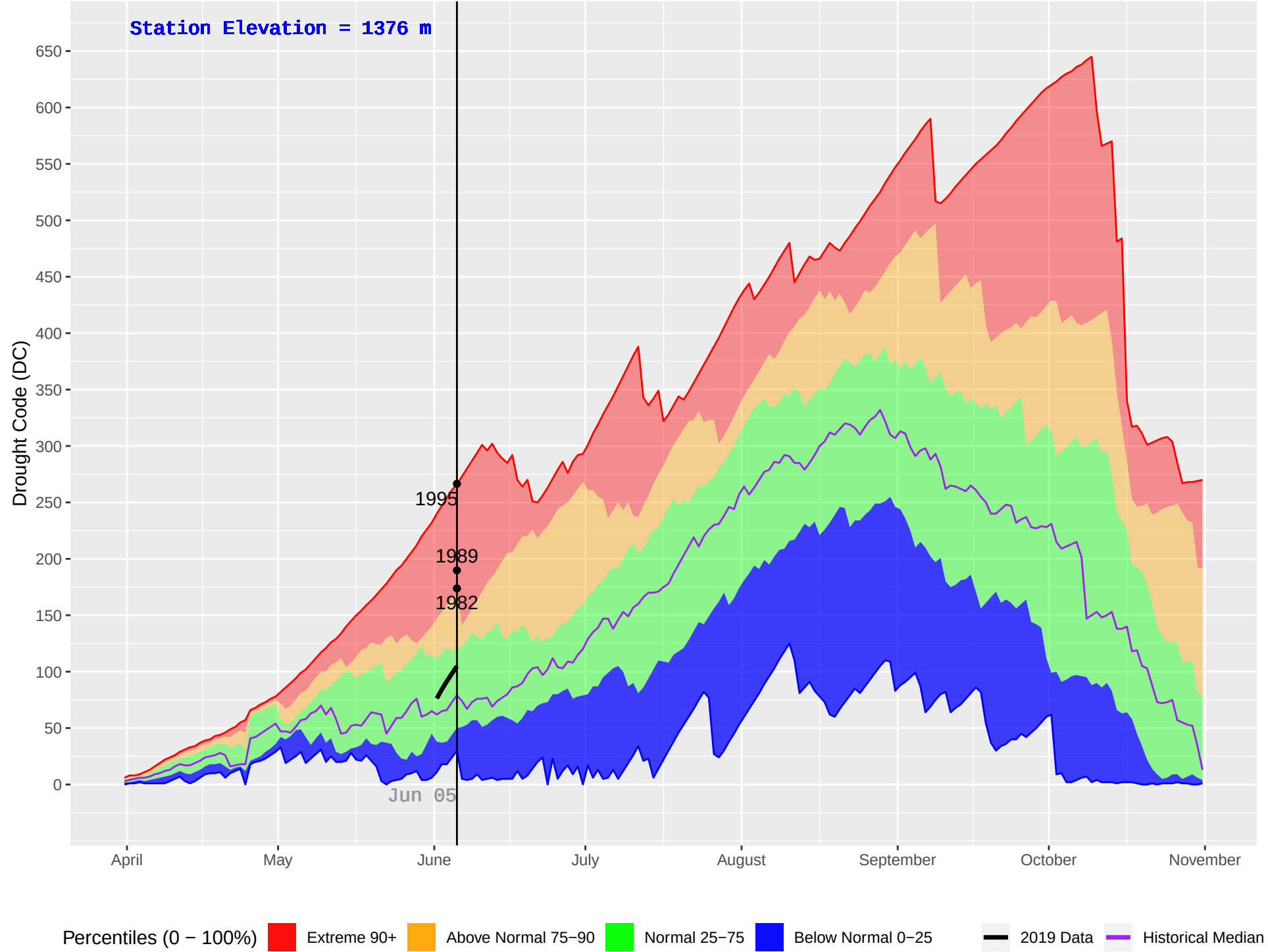
DUNCAN (385) : Historical (1981–2018) and Current (2019) Daily Drought Code (DC)
