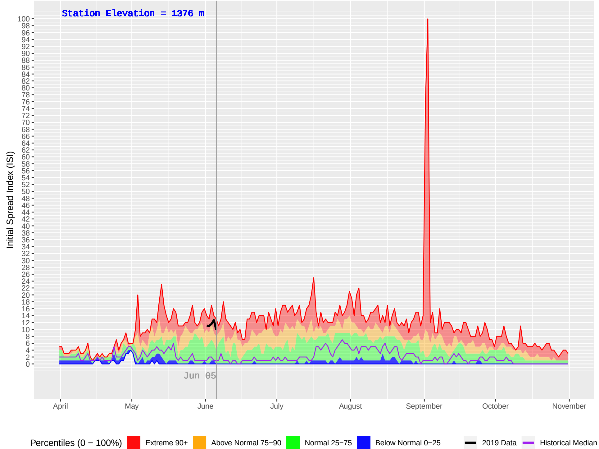
DUNCAN (385) : Historical (1981–2018) and Current (2019) Daily Initial Spread Index (ISI)
