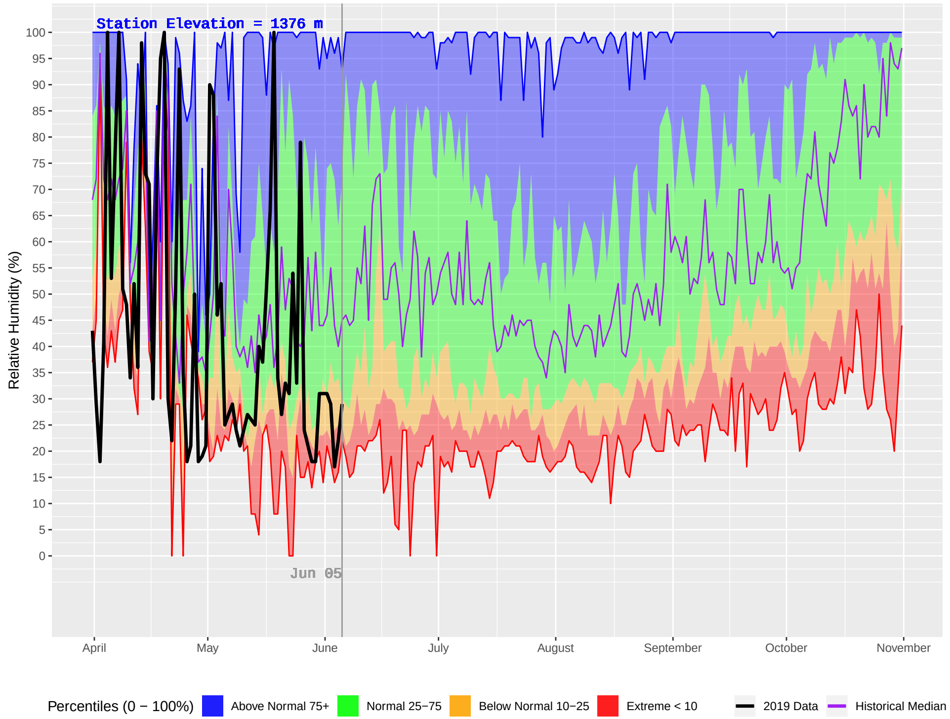
DUNCAN (385) : Historical (1981–2018) and Current (2019) Daily Relative Humidity
