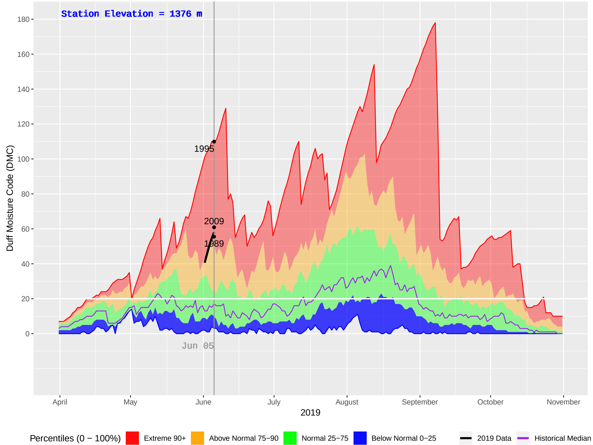
DUNCAN (385) : Historical (1981–2018), Current (2019) Daily Duff Moisture Code (DMC)
