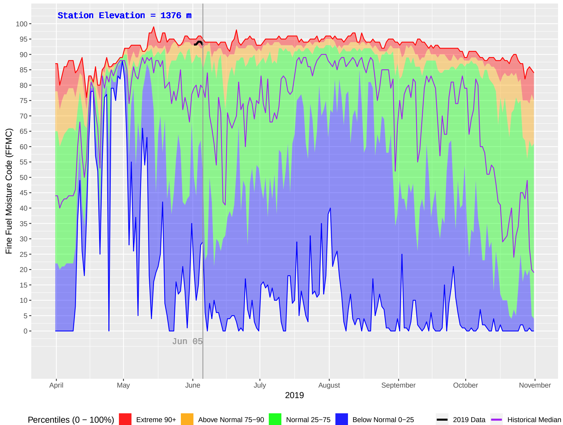
DUNCAN (385) : Historical (1981–2018) and Current (2019) Daily Fine Fuel Moisture Code (FFMC)
