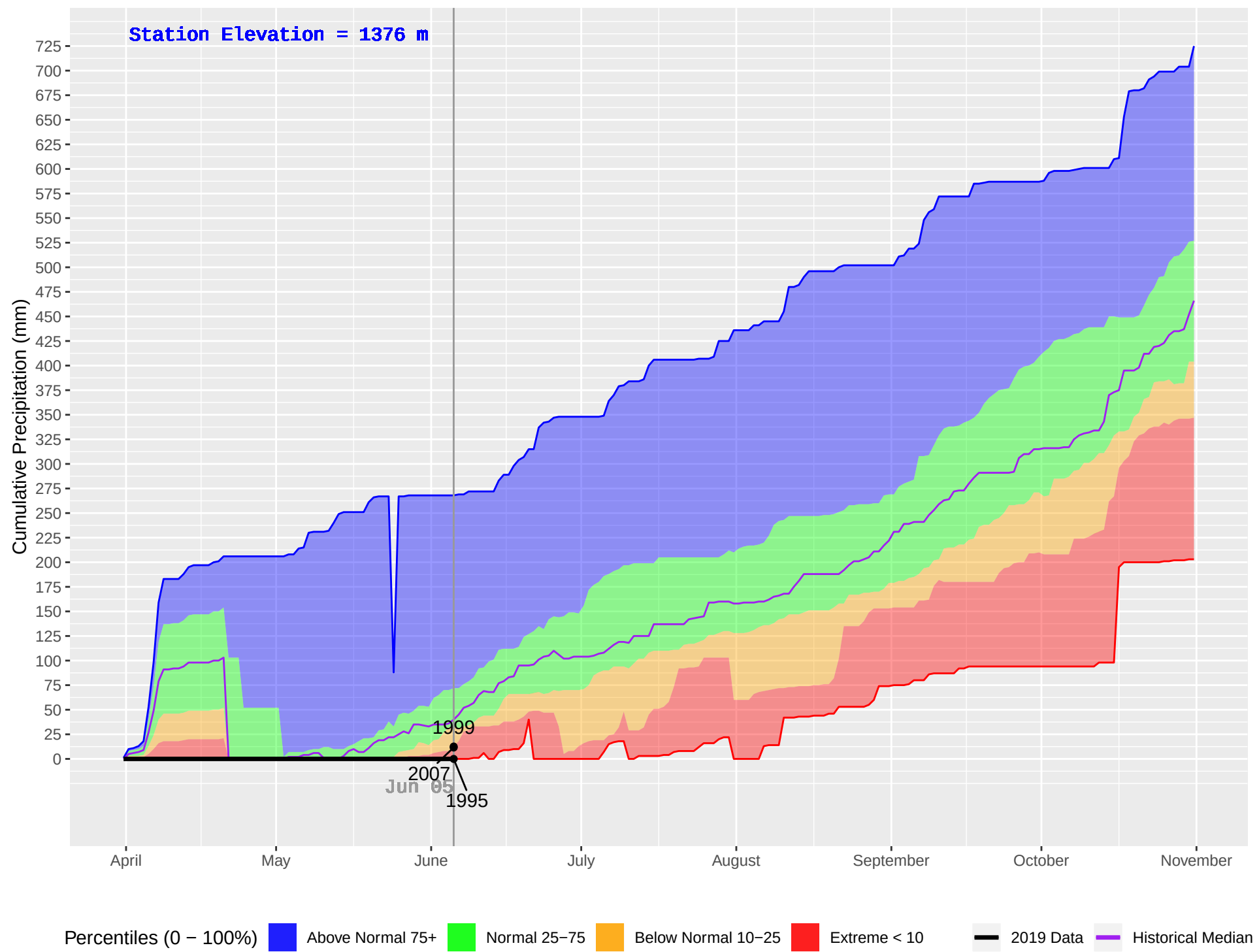
DUNCAN (385) : Historical (1981–2018), Current (2019) Daily Cumulative Precipitation
