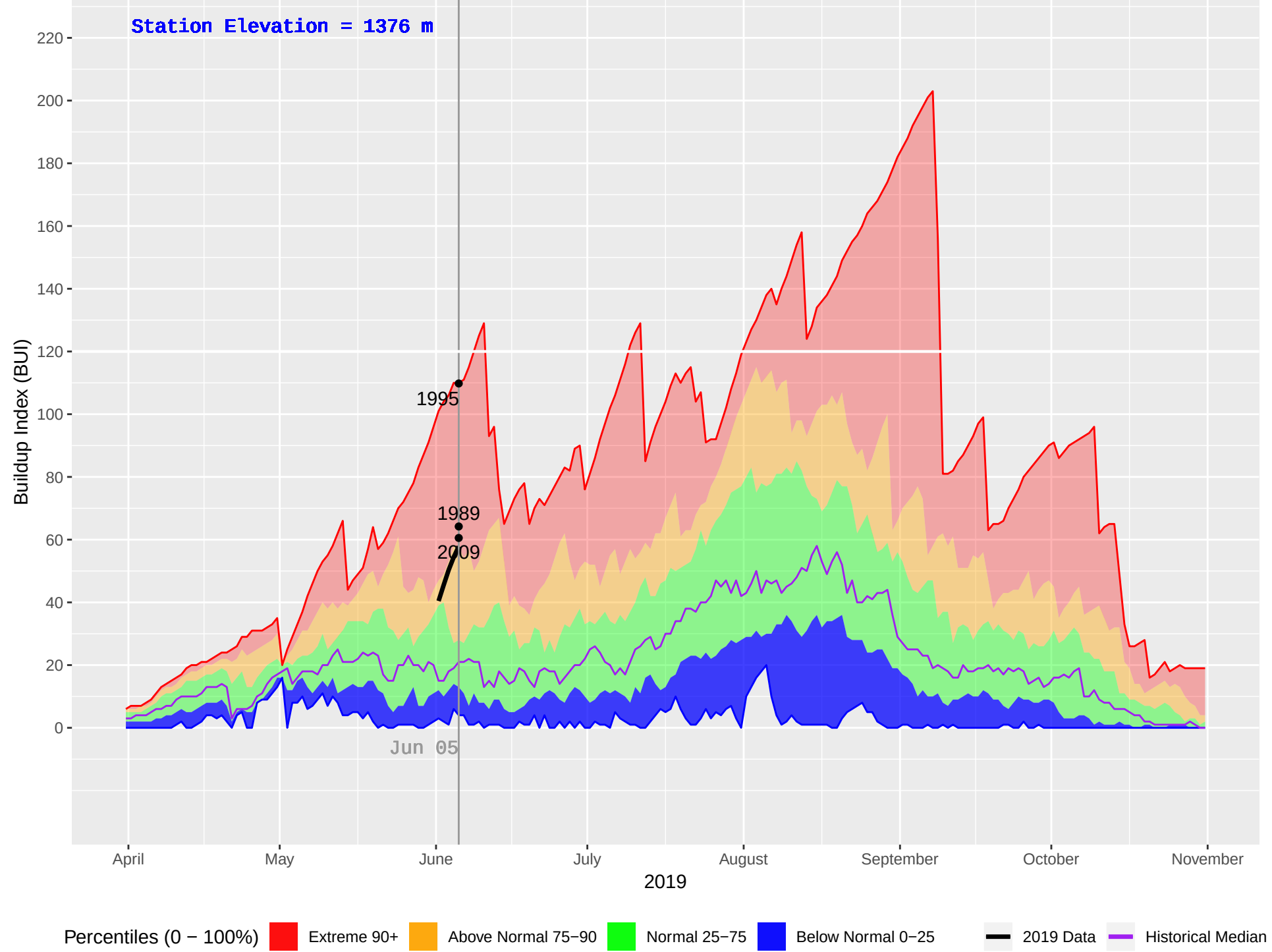
DUNCAN (385) : Historical (1981–2018), Current (2019) Daily Buildup Index (BUI)
