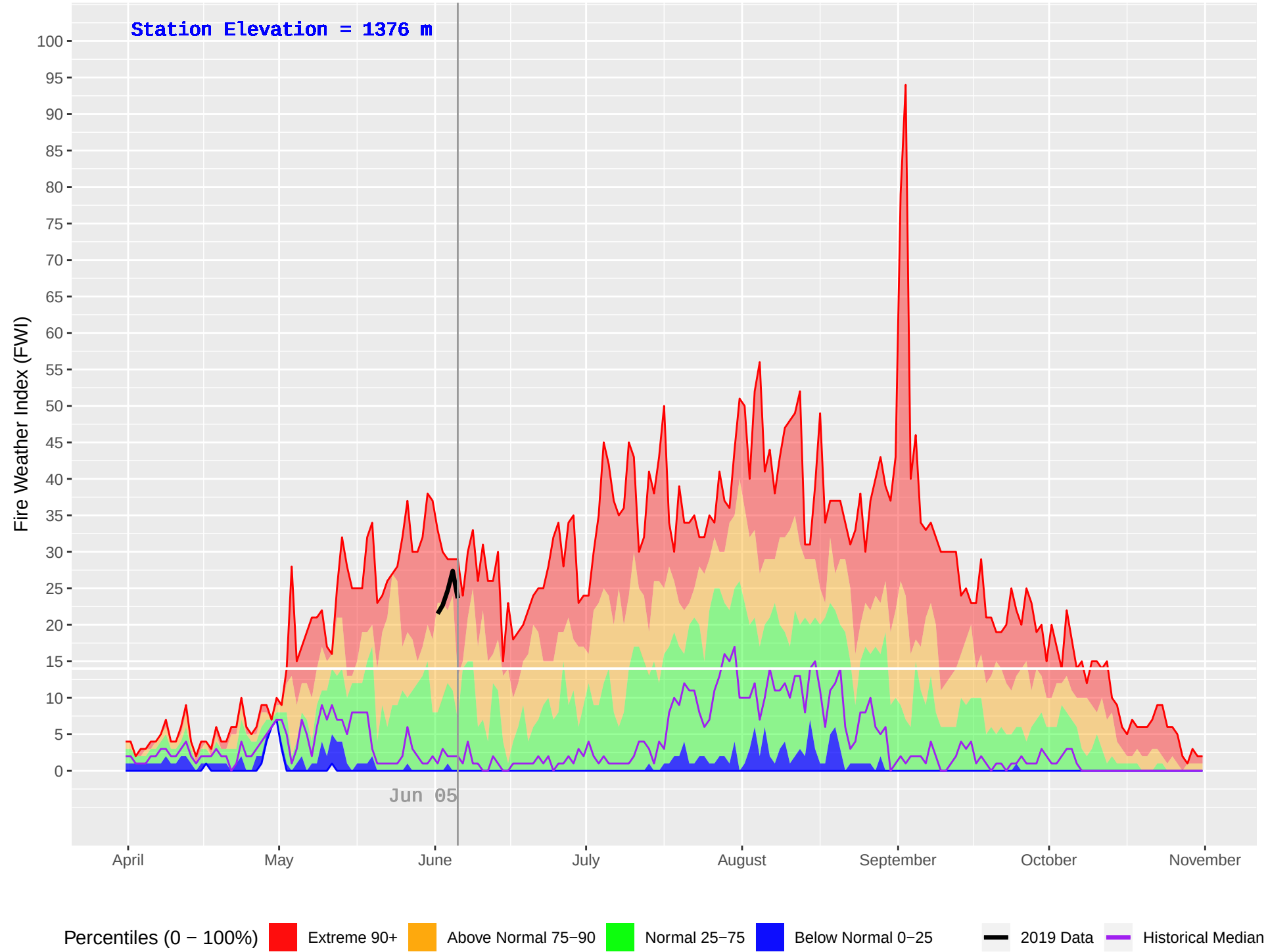
DUNCAN (385) : Historical (1981–2018) and Current (2019) Daily Fire Weather Index (FWI)
